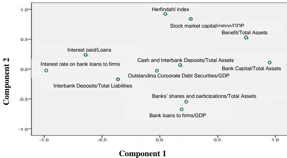
Figure 1 Correlations of the principal components with the original variables
